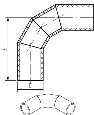
pipe segments
