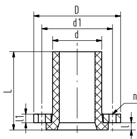
socket welding
