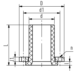
socket welding
