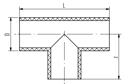
Injection molded fitting
